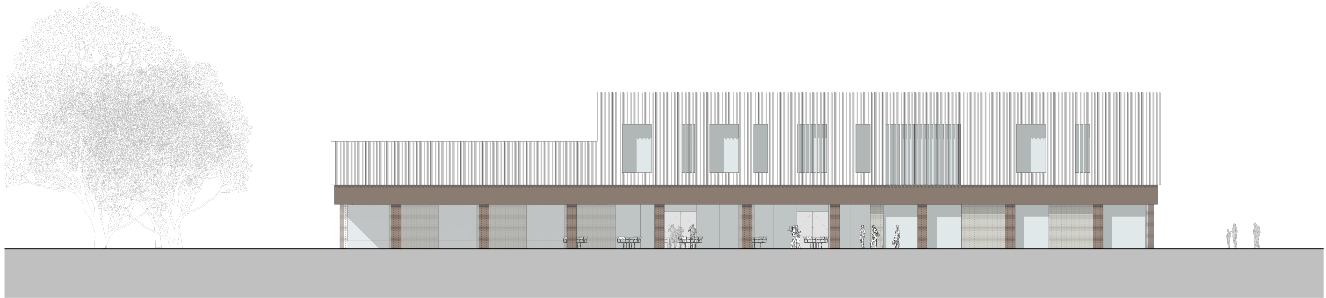
Elevation Project South
